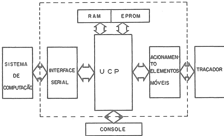
FIG. 1- INTERFACE
